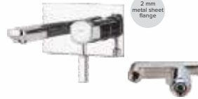
Wall mounted single lever basin mixer with 2 mm sheet flange Exposed part F1014474 ₹ 4,240 Concealed part F4065103 ₹ 3,050 Set ₹ 7,290
